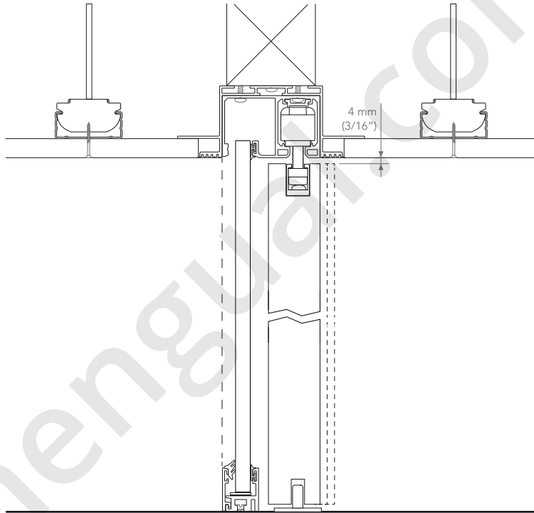
EMPOTRADO / RECESSED
