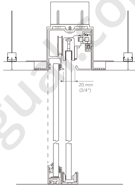
EMPOTRADO / RECESSED
