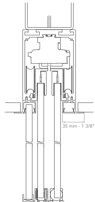
EMPOTRADO / RECESSED
