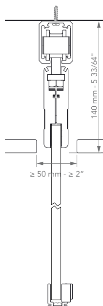
EMPOTRADO / RECESSED
