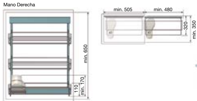
Base zapatero
